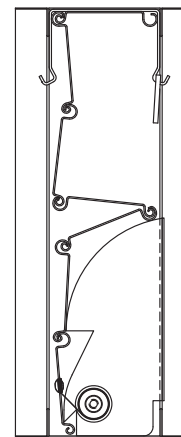
Closed Position (D37V)
